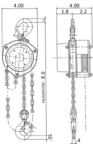
Above schematic measured in inches
